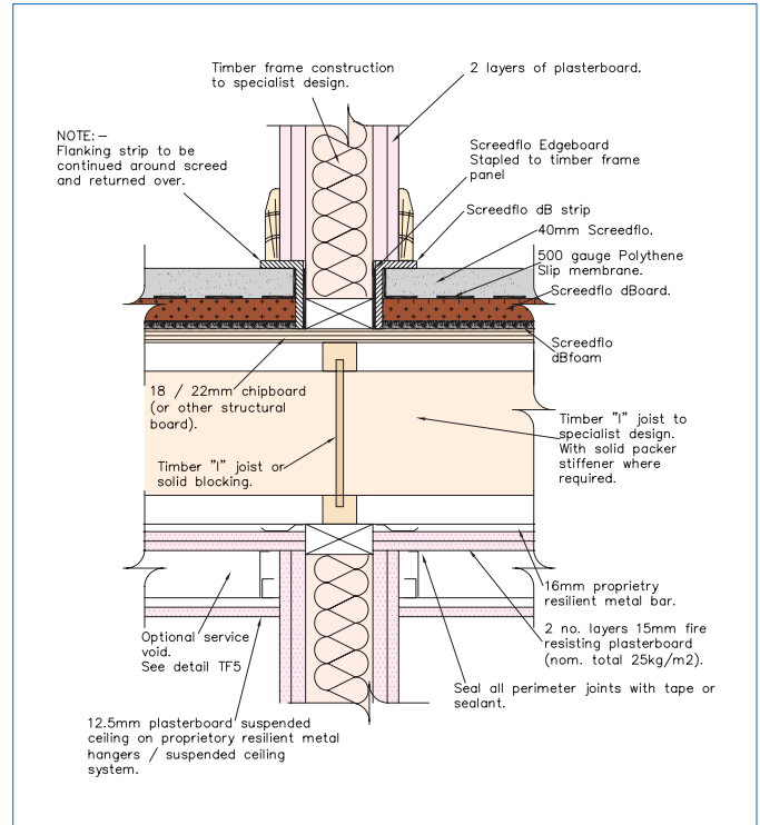
Fig 3: Load bearing wall
