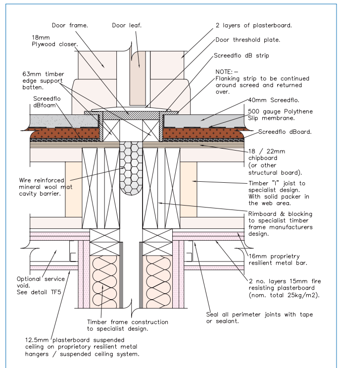
Fig 4: Door thresholds
