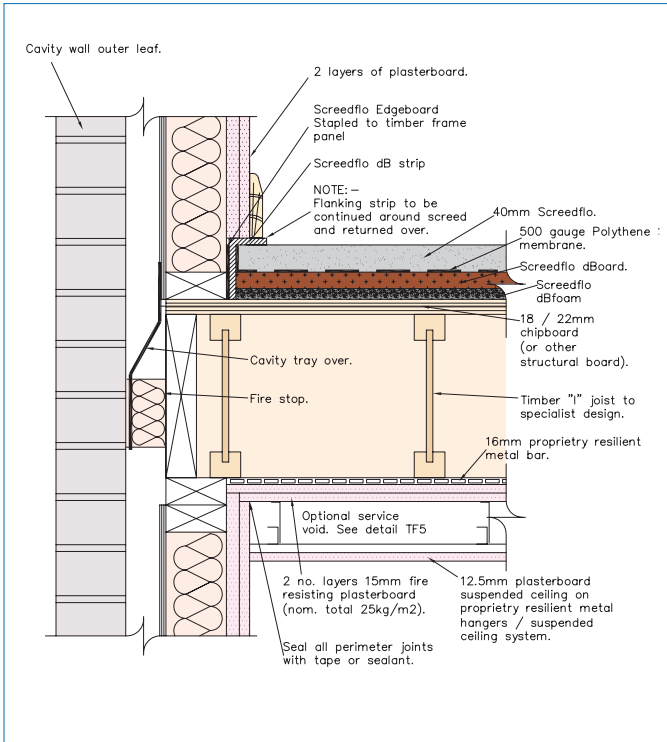
Fig 1: External wall junction
