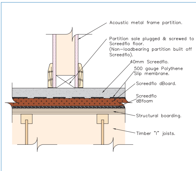
Fig 2: Non-load bearing partition
